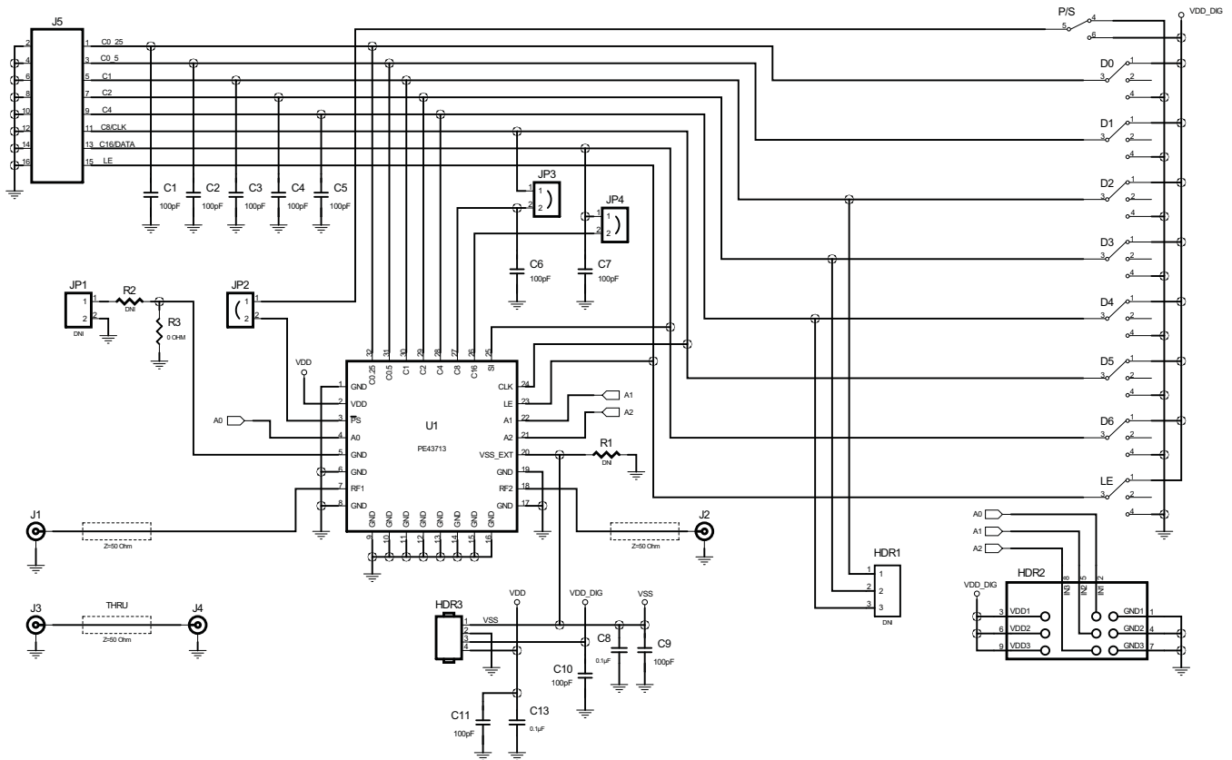
Figure 13 • PE43713 Evaluation Board Schematic
