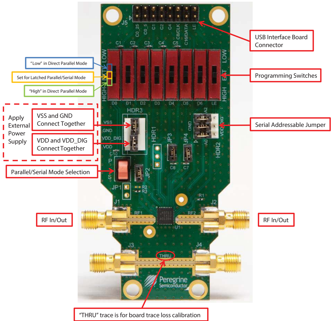
Figure 14 • PE43713 Evaluation Board Outline Showing Functional Overview
