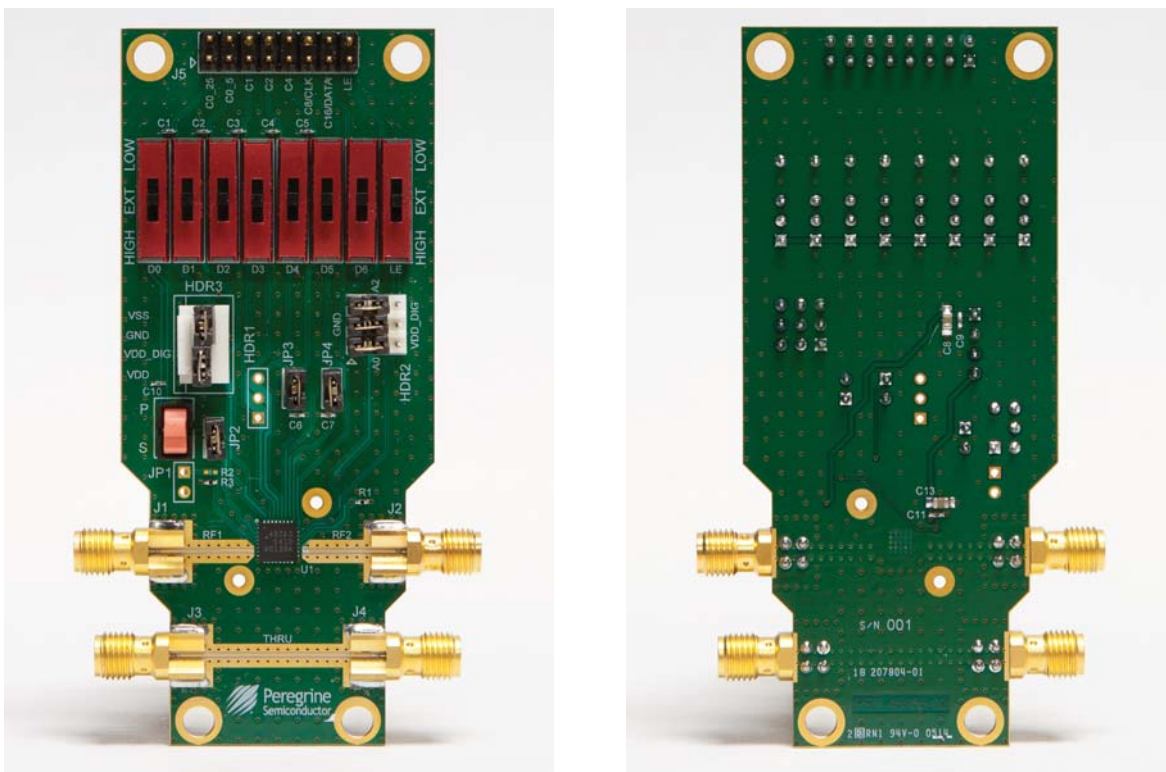
Figure 1 • PE43713 Evaluation Board Assembly
