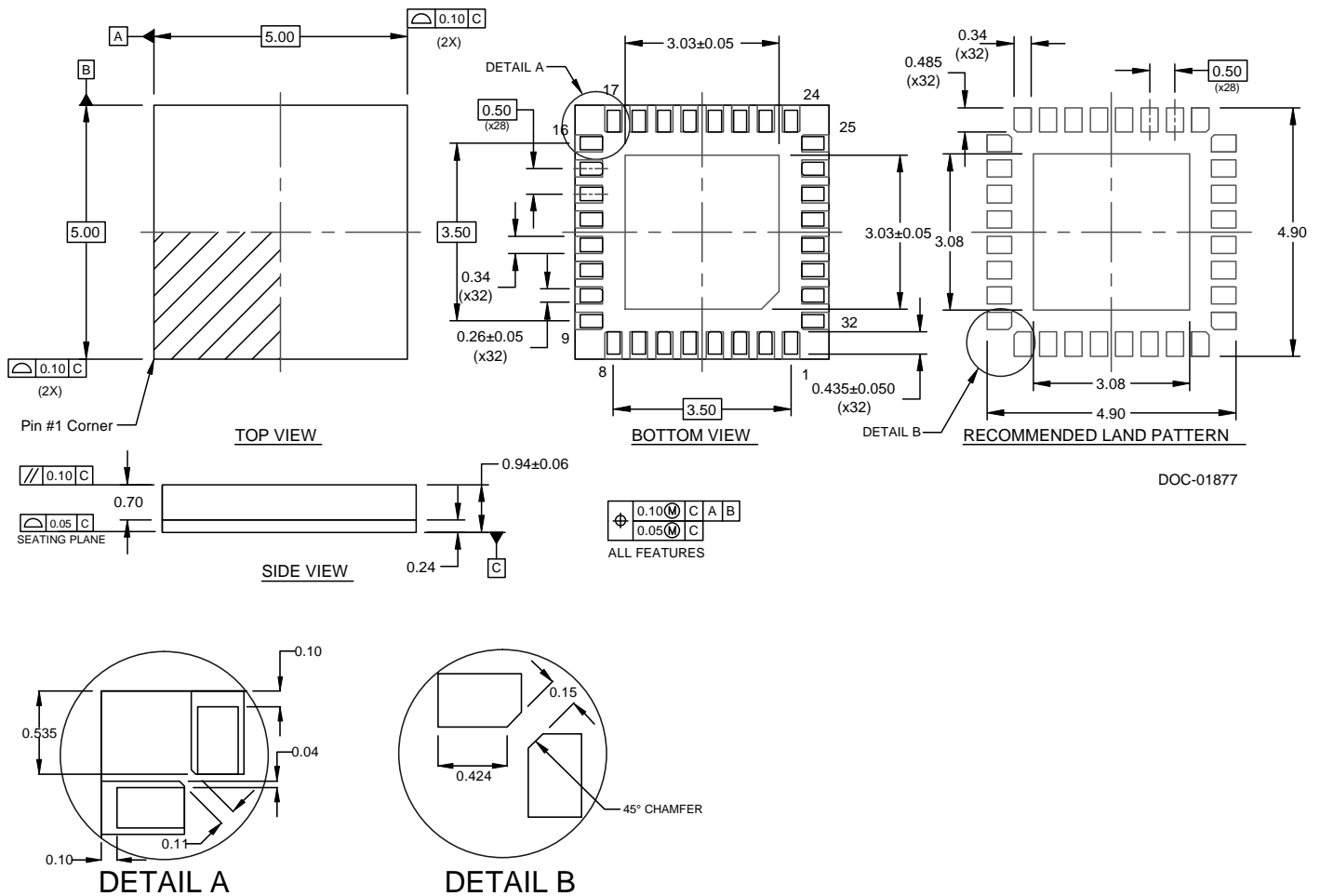
Figure 21. Package Drawing
