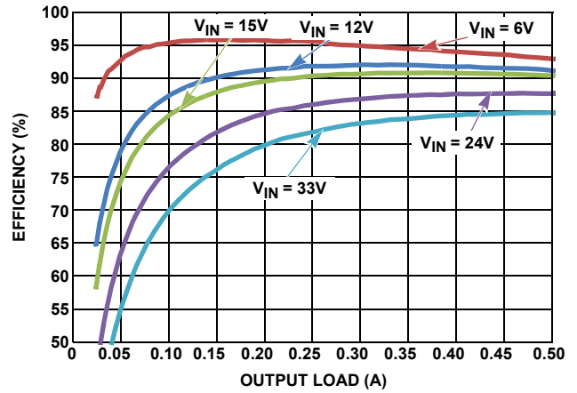
FIGURE 6. EFFICIENCY vs LOAD, PWM, V_{OUT} = 5\text{V}
