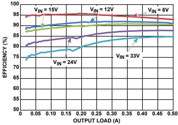
FIGURE 5. EFFICIENCY vs LOAD, PFM, V_{OUT} = 5\text{V}
